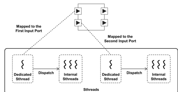
[Fig. 1] Process and its sthreads
